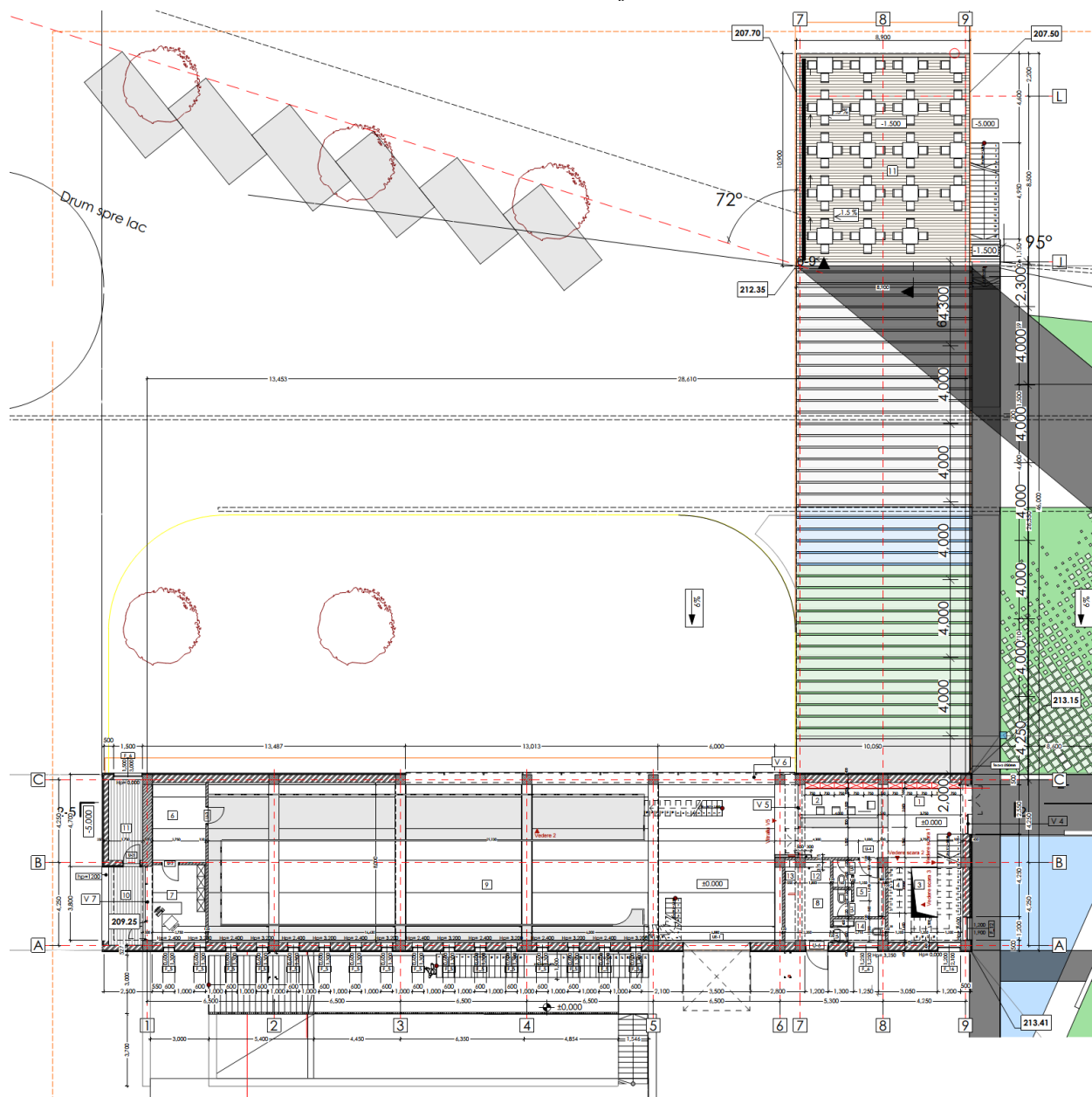
Figura A4.89. Plan parter, cota \pm 0.000
