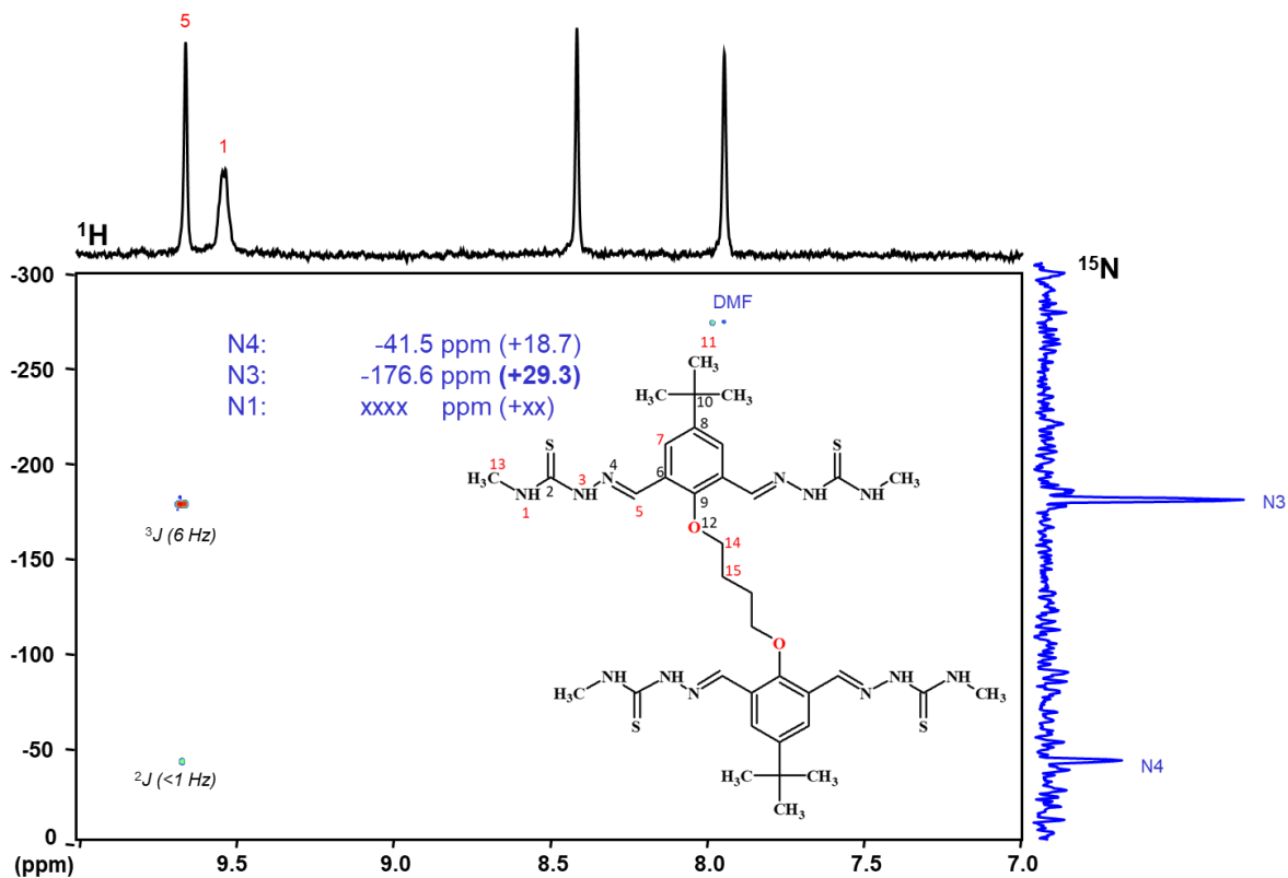
Fig. A10.18 400 MHz ^1\text{H}\{^{15}\text{N}\} HMBC RMN (DMSO- d_6 ) spectrum of [(\text{Mo}_2\text{O}_2\text{S}_2)_2(\text{L}^{20})]
