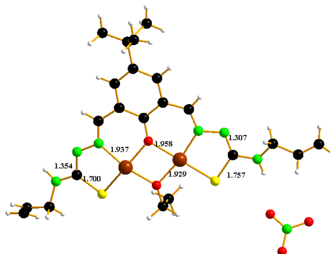
Fig. 4.35. Structura moleculară a compusului [\text{Cu}_2(\text{HL}^{18})\text{OC}_2\text{H}_5]\text{NO}_3
