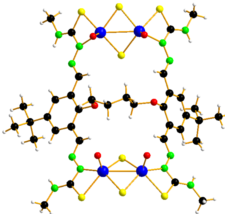
Fig. 4.22. Structura moleculară a compusului [(\text{Mo}_2\text{O}_2\text{S}_2)_2(\text{L}^{20})]
