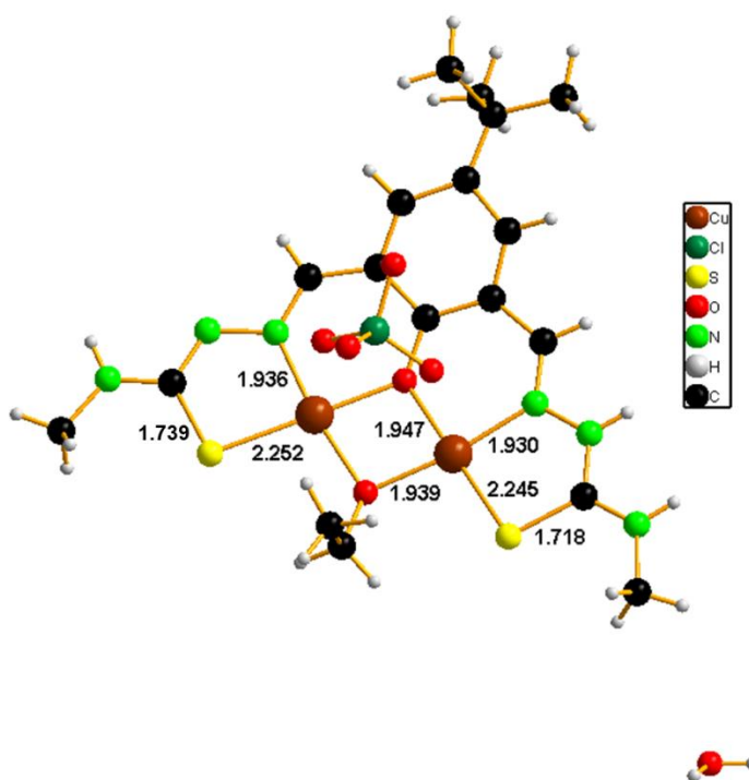
Fig. 4.37. Structura moleculară a compusului [\text{Cu}_2(\text{HL}^{16})\text{OC}_2\text{H}_5]\text{ClO}_4
