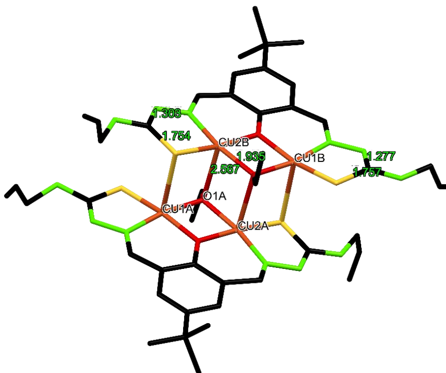
Fig. 4.34. Packing-ul compusului [\text{Cu}_2(\text{L}^{18})\text{OC}_2\text{H}_5]
