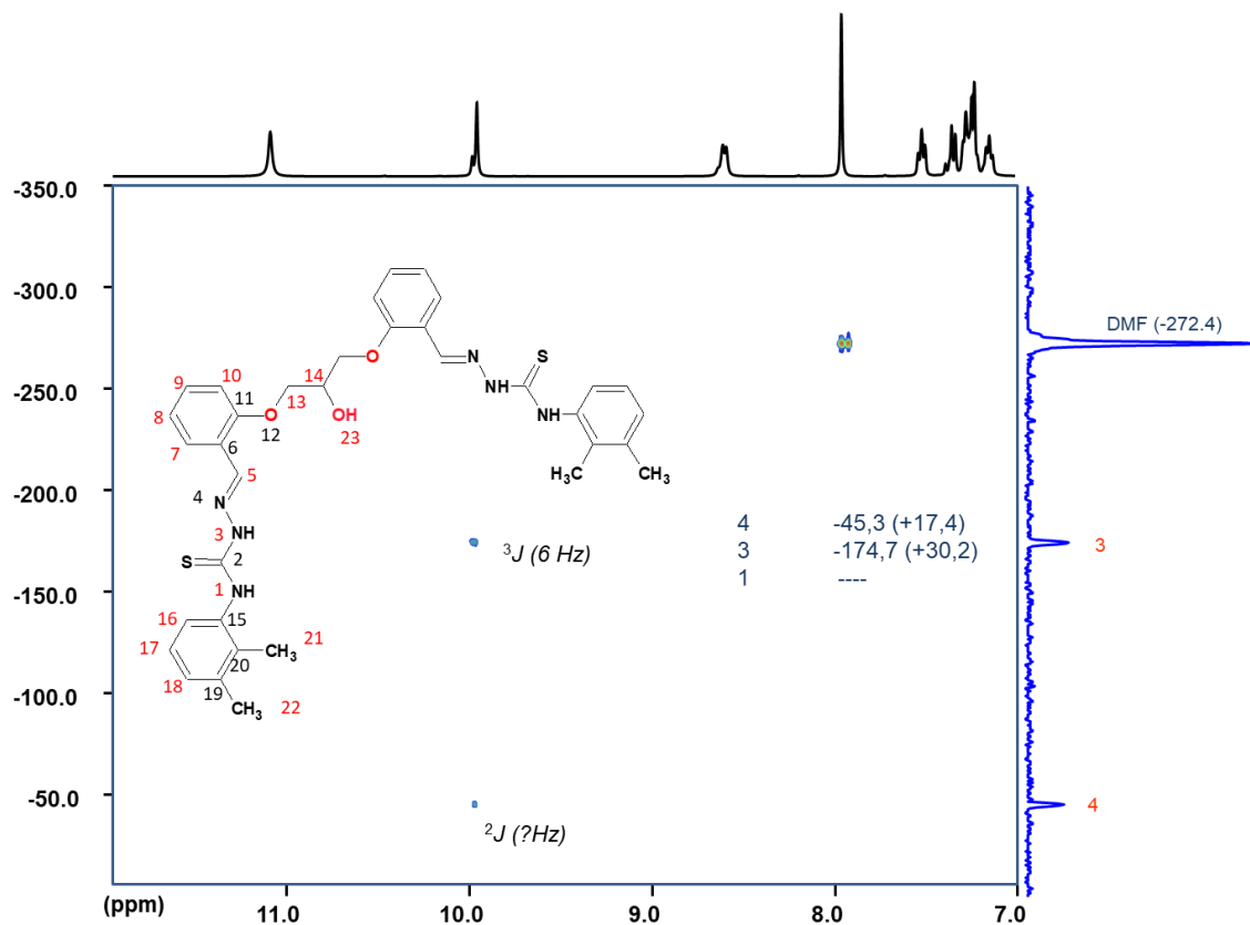
Fig. A10.8 400 MHz ^1H\{^{15}N\} HMBC RMN (DMSO- d_6 ) spectru al [Mo_2O_2S_2(HL^{10})]
