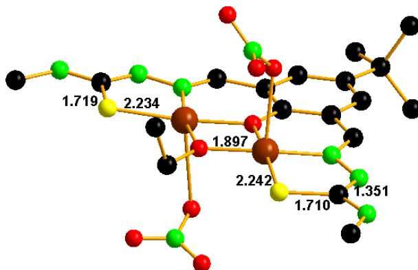
Fig. 4.38. Structura moleculară a compusului [\text{Cu}_2(\text{H}_2\text{L}^{16})\text{OC}_2\text{H}_5(\text{NO}_3)_2]
