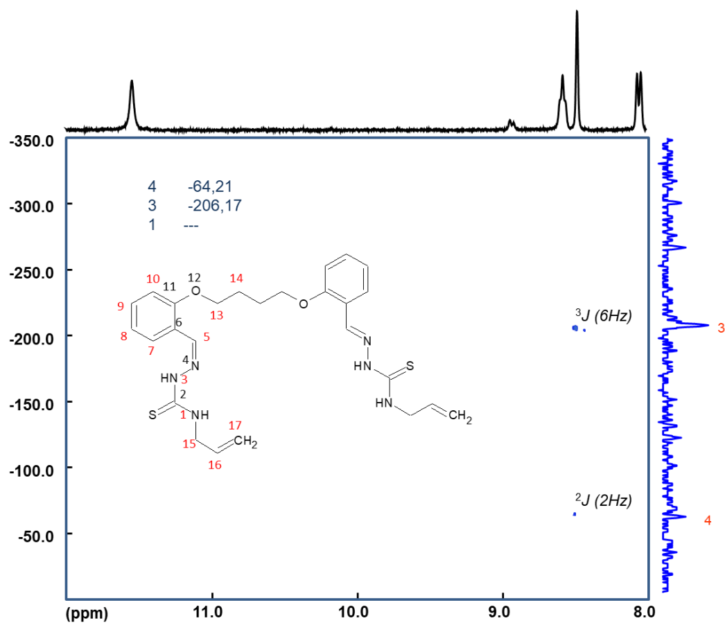
Fig. A10.3 400 MHz ^1H\{^{15}N\} HMBC RMN (DMSO- d_6 ) spectru al H_2L^8
