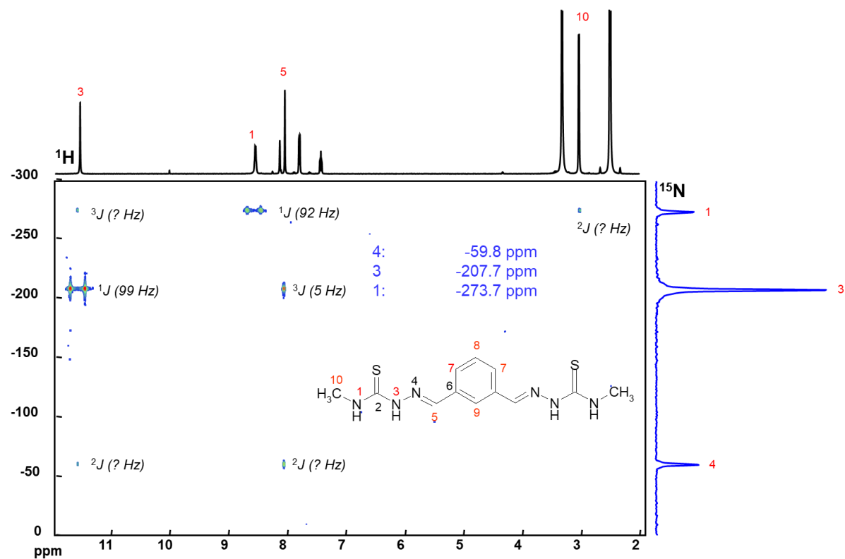
Fig. A10.12 400 MHz ^1\text{H}\{^{15}\text{N}\} HMBC RMN (DMSO- \text{d}_6 ) spectru al H 2 L 14
