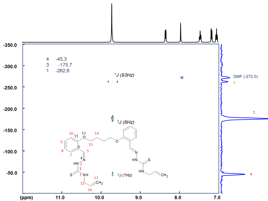
Fig. A10.4 400 MHz ^1H\{^{15}N\} HMBC RMN (DMSO- d_6 ) spectru al [Mo_2O_2S_2(L^8)]
