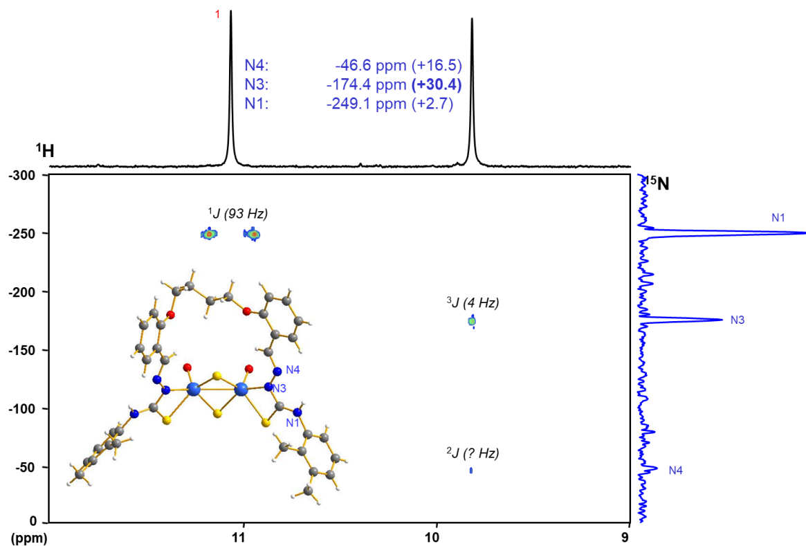
Fig. A10.1 400 MHz ^1\text{H}\{^{15}\text{N}\} HMBC RMN (DMSO- \text{d}_6 ) spectru al \text{H}_2\text{L}^7
