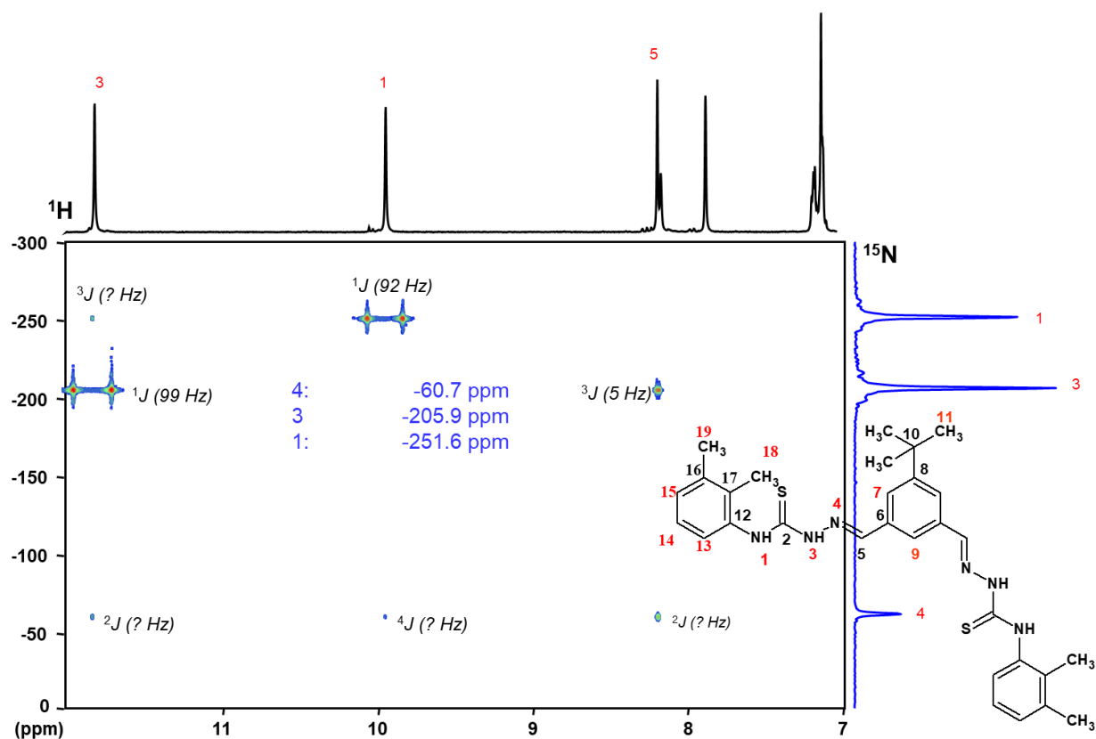
Fig. A10.11 400 MHz ^1\text{H}\{^{15}\text{N}\} HMBC RMN (DMSO- \text{d}_6 ) spectru al H 2 L 13
