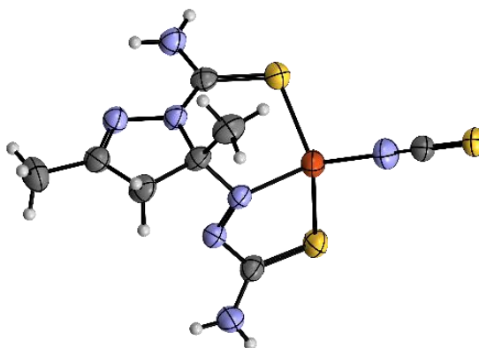
Fig. 1.20. Structura cristalină a complexului [(\text{L}^{\text{va}})\text{Cu}(\text{NCS})] CCDC 2022923 [58]
