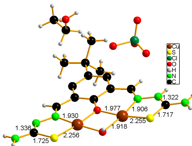
Fig. 4.36. Structura moleculară a compusului [\text{Cu}_2(\text{HL}^{15})\text{OH}]\text{ClO}_4
