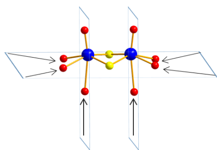
Cluster [\text{Mo}_2\text{O}_2\text{S}_2(\text{H}_2\text{O})_6]^{2+}
