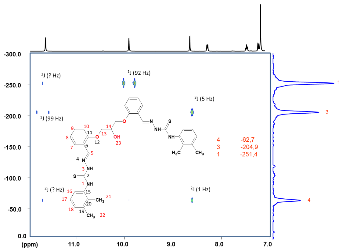
Fig. A10.7 400 MHz ^1H\{^{15}N\} HMBC RMN (DMSO- d_6 ) spectru al H_3L^{10}
