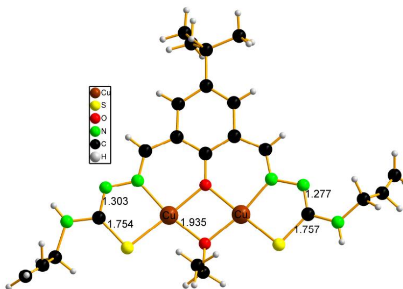
Fig. 4.33. Structura moleculară a compusului [\text{Cu}_2(\text{L}^{18})\text{OC}_2\text{H}_5]
