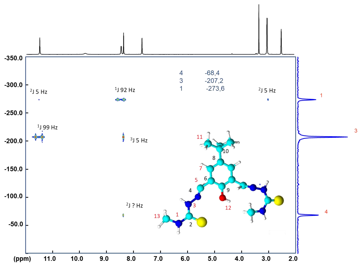
Fig. A10.14 400 MHz ^1H\{^{15}N\} HMBC RMN (DMSO- d_6 ) spectru al H_3L^{16}
