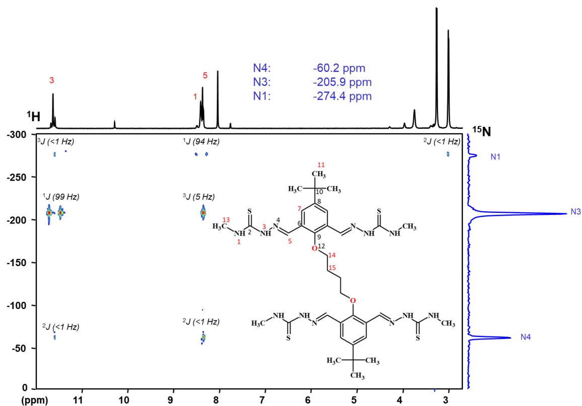
Fig. A10.17 400 MHz ^1\text{H}\{^{15}\text{N}\} HMBC RMN (DMSO- d_6 ) spectrum of \text{H}_4\text{L}^{20}
