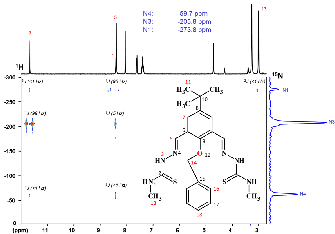
Fig. A10.15 400 MHz ^1\text{H}\{^{15}\text{N}\} HMBC RMN (DMSO- \text{d}_6 ) spectrum of \text{H}_2\text{L}^{19}
