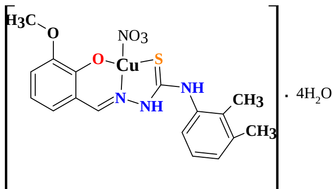
Fig. 1.23. Structura complexului [\text{Cu}(\text{HL}^{\text{caa}})\text{NO}_3] \cdot 4\text{H}_2\text{O}
