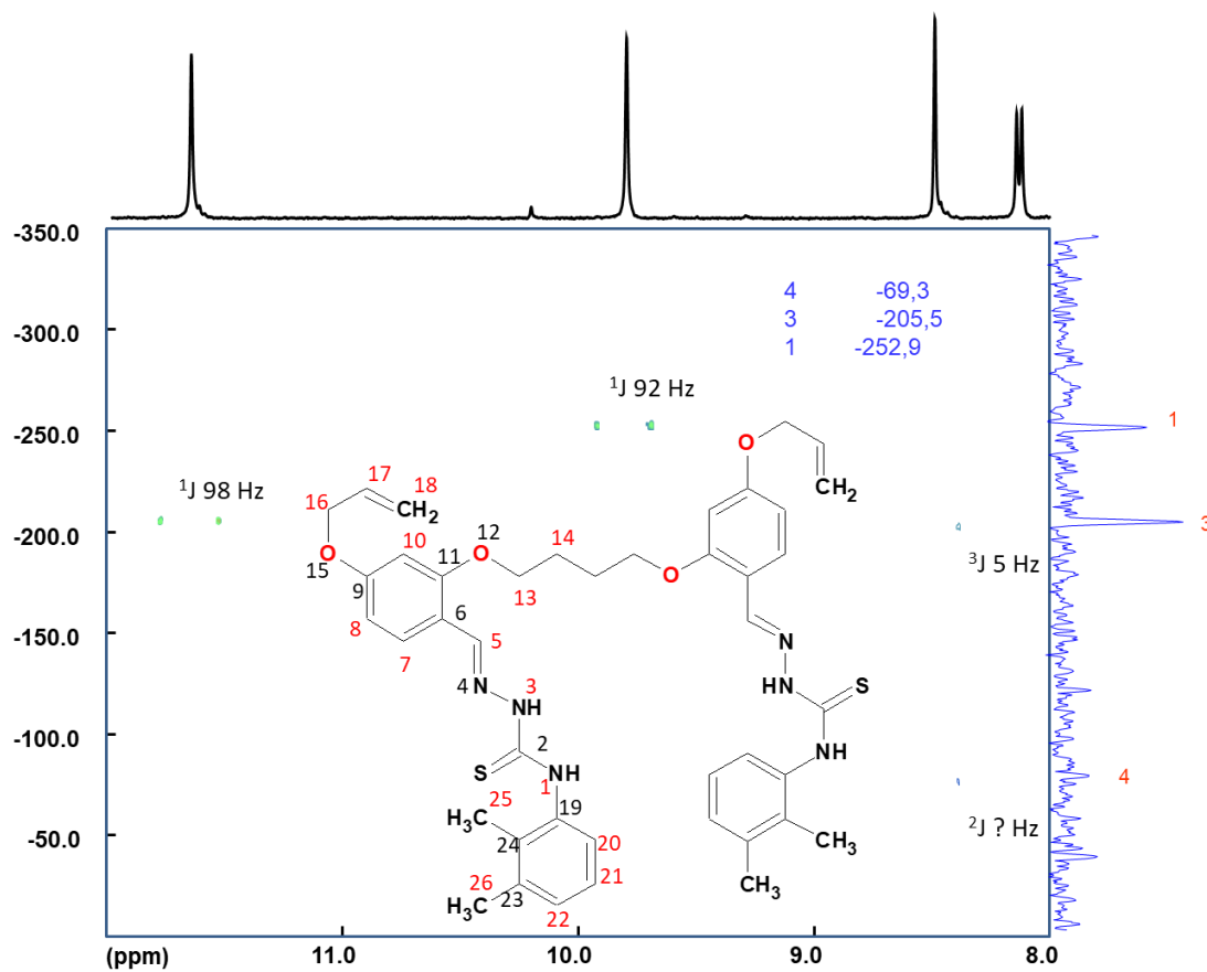
Fig. A10.5 400 MHz ^1H\{^{15}N\} HMBC RMN (DMSO- d_6 ) spectru al H_2L^9
