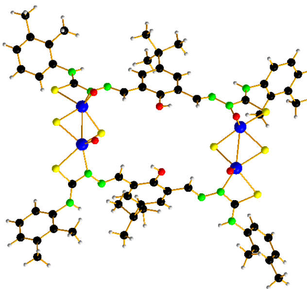
Fig. 4.21. Structura moleculară a compusului [\text{Mo}_2\text{O}_2\text{S}_2(\text{HL}^{17})]_2
