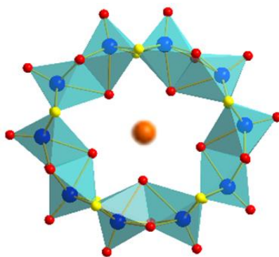
Fig. 2.9. Structura precursorului \text{K}_{2-x}(\text{NMe}_4)_x[\text{I}_2\text{Mo}_{10}\text{O}_{10}\text{S}_{10}(\text{OH})_{10}(\text{H}_2\text{O})_5] [80]
