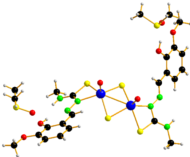
Fig. 3.8. Structura moleculară a complexului [\text{Mo}_2\text{O}_2\text{S}_2(\text{HL}^3)_2] \cdot 2\text{DMSO}
